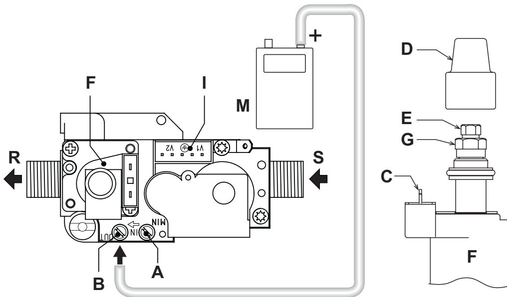
fig. 23 - Valvola gas
